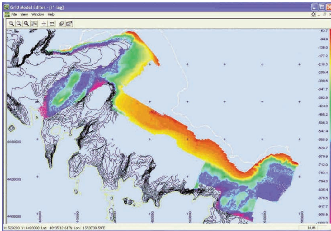
Figure 3 Total coverage map of the Multibeam acquisition during the oceanographic cruise SISTERII. The visualization of the bathymetric data has been realised through a colorimetric scale and using the software PDS2000 (RESON; navigation and Multibeam acquisition).
