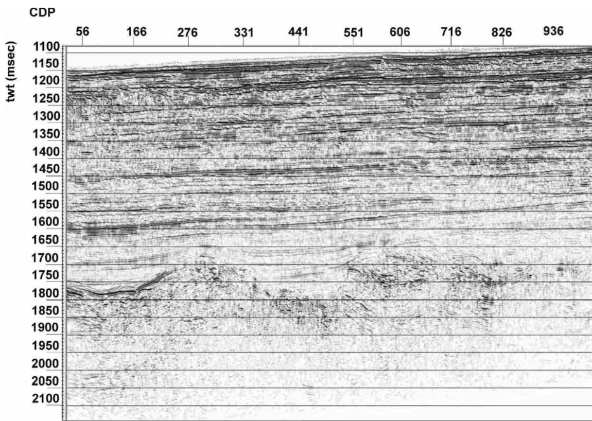
Figure 25 Detail of the multichannel seismic profile L6 showing the Meso-Cenozoic unconformity. Figura 25 Dettaglio del profilo sismico multicanale L6 mostrandente la unconformity meso-cenozoica.
